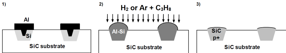
Figure 1: Schematic description of the localized VLS epitaxy process: 1) deposition of Al-Si stack inside the trenches / bowls formed by ICP in SiC, 2) melting of Al-Si and addition of propane for the VLS growth, 3) selective formation of P + -type SiC
