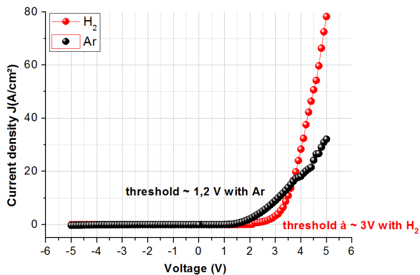
Figure 3 : Current-voltage characteristics in forward bias for P/N junctions in which P + material was grown by VLS : Ar carrier gas (●) vs H 2 carrier gas (●)
