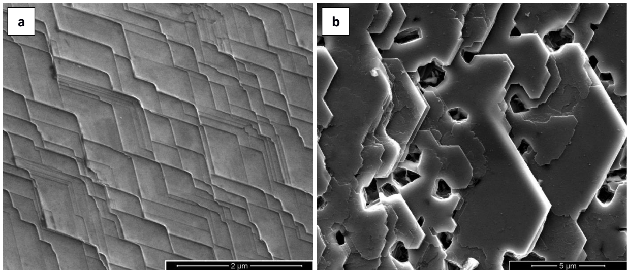
Figure 2 : Surface morphology after etching the remaining alloy on samples grown by VLS : under H 2 carrier gas (a - left), and under Ar carrier gas (b - right)
