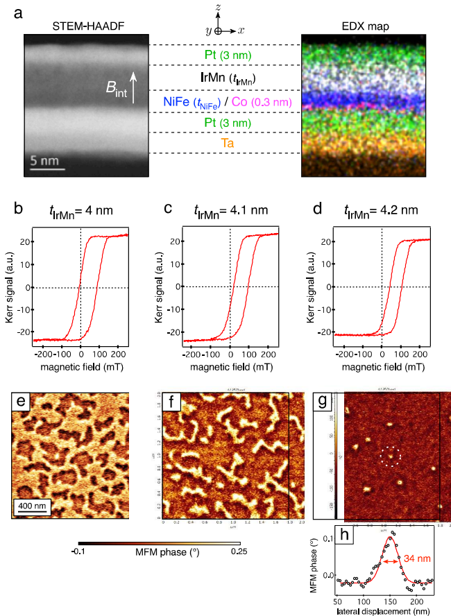
FIG. 1: (a) Central panel: Schematic structure of the exchange-biased multilayer stack. Left panel: Scanning transmission electron microscopy image of a cross-section of the sample obtained in a high-angle annular dark-field imaging (STEM-HAADF) mode. Right panel: energy-dispersive X-ray (EDX) elemental map. The white arrow indicates the direction of the internal exchange bias field B_{\text{int}} across the NiFe/IrMn interface. (b-d) Magneto-optical Kerr rotation recorded as a function of a magnetic field applied perpendicularly to the film plane for various IrMn thicknesses, (b) t_{\text{IrMn}} = 4 nm, (c) t_{\text{IrMn}} = 4.1 nm and (d) t_{\text{IrMn}} = 4.2 nm. For these experiments, the NiFe thickness is t_{\text{NiFe}} = 2.1 nm. (e-g) Corresponding magnetic force microscopy (MFM) images recorded at zero external magnetic field. (h) Line profile across the skyrmion marked with the white dashed circle in (g). The red solid line is a Gaussian fit, leading to a full width at half maximum w_{\text{MFM}} = 34 \pm 3 nm.
