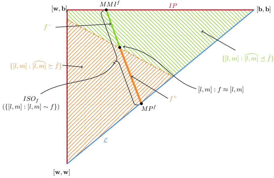
Figure 3: Illustration of \mathcal{B} and the construction in the proof of Lemma A.2
