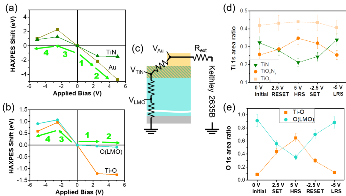
Figure 2. (a) HAXPES shift of Au 4f, Ti 1s and (b) O 1s depending on the applied voltage (c) equivalent circuit of the structure with R_{ext} = 2.9 \Omega (d) relative areas of all Ti 1s and (e) O 1s contributions depending on the applied bias and the resistance state
