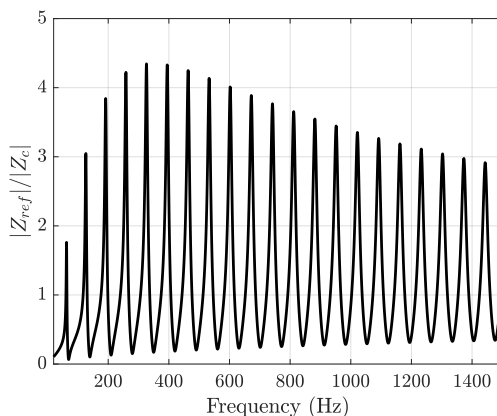
Figure 2: Reference input impedance of the simplified bassoon computed by a division in 10^5 conical frustums with ZK-losses computed with Eqs.(22) and (23) for the equivalent radius R_n^{eq} of each conical frustum (Eq.(43)).
