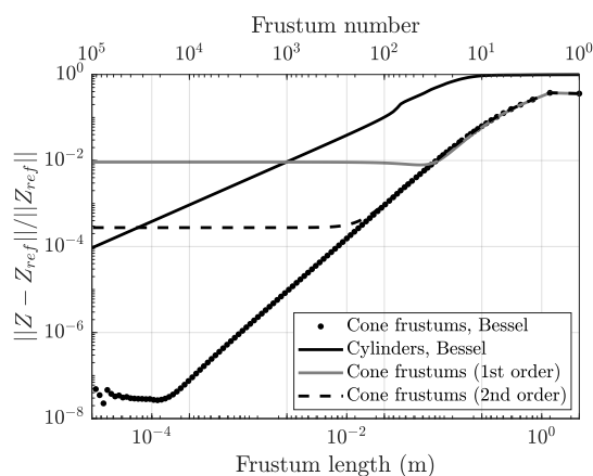
Figure 3: Evolution of the norm of the relative difference with the reference impedance Z_{ref} ( 10^5 conical frustums with ZK-losses) versus the length of each frustum for different approximations (Cylinders with ZK-losses, conical frustums with ZK-losses, 1st or 2nd order approximation of losses).
