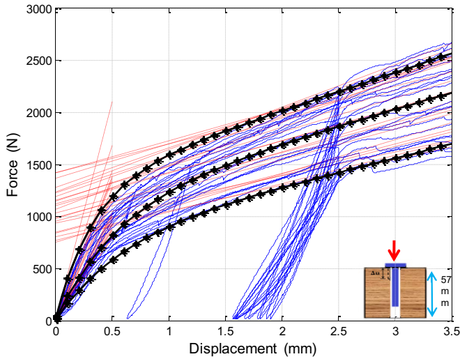
Fig. 8. Screw compression in wood test and results.
