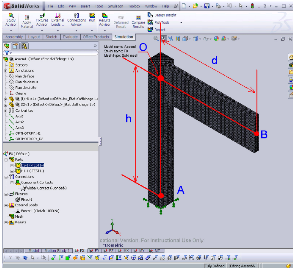
Fig. 1. Screen shot of the CAD model of the corner. Lengths are h = 447 m and d = 428.5 mm. Sectional areas are 57 \times 57 mm 2 edge for the vertical part and 20 \times 140 mm 2 for the horizontal one. All dof are naught in section A and loads are applied in section B.
