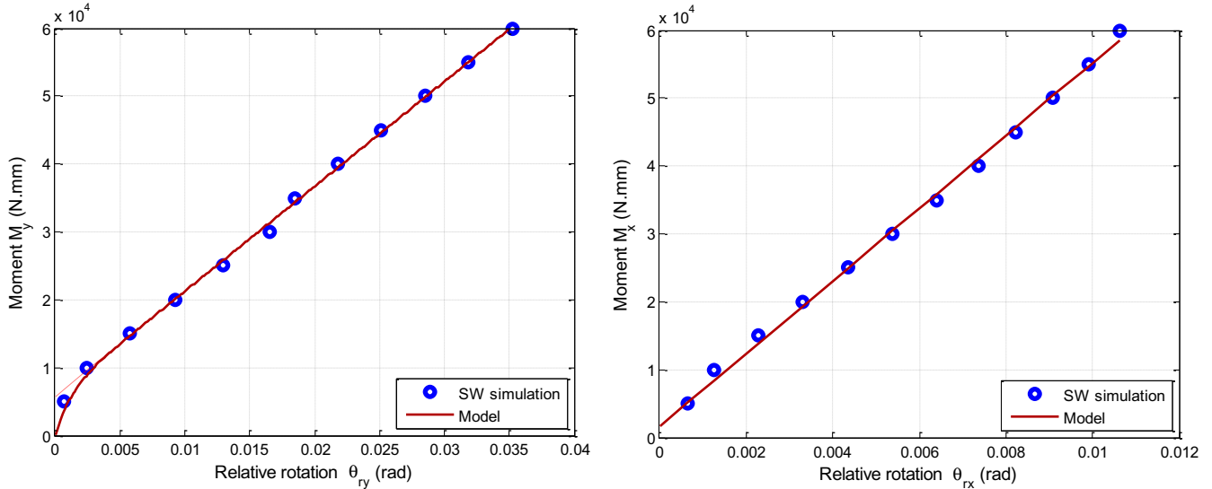
Fig. 4. Spring rotational behavior, k_{\theta_x} and k_{\theta_y} stiffnesses.
