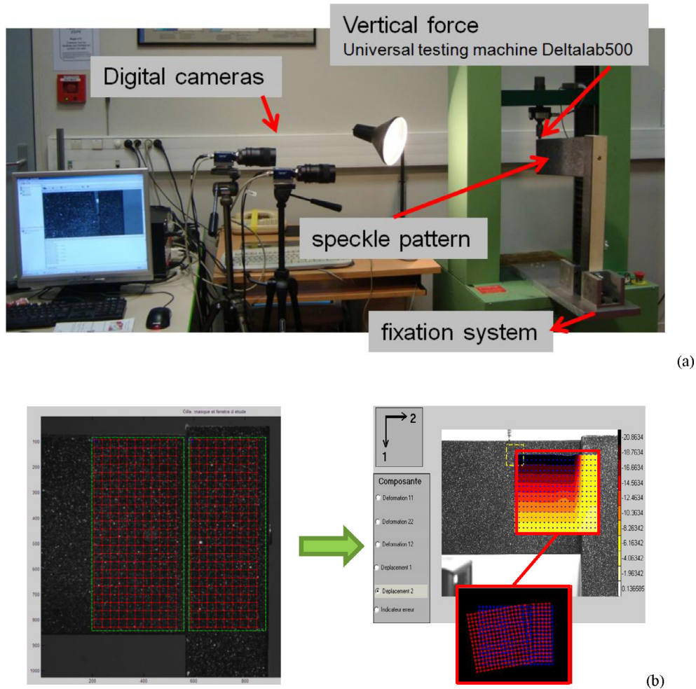
Fig. 6. Presentation of the corner test experiment (a) details on the apparatus (b) angle gap \theta_{rz} measurement with DIC.
