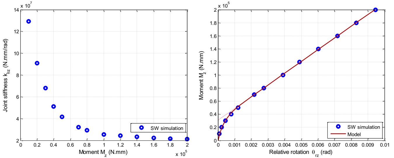
Fig. 3. Left, stiffness vs. moment and right, moment vs. relative rotation (results and model).
