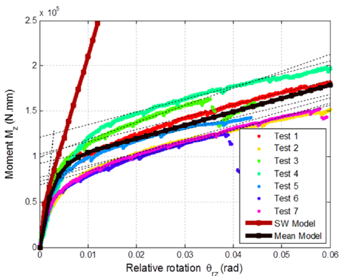
Fig. 7. M_z versus \theta_{rz} curves compared with the FEA curve – dots are direct measurement obtained from the displacement of the testing machine and the line is obtained from 3D finite element simulation.
