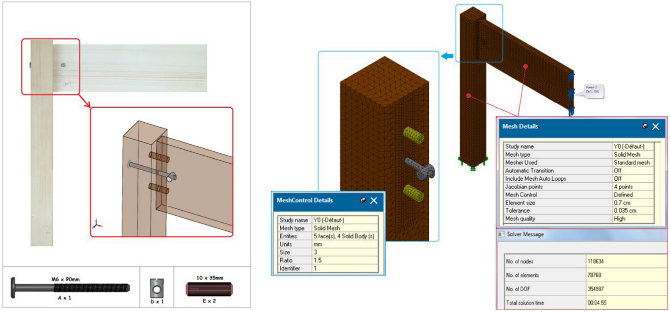
Fig. 2. CAD and meshing of the “real” corner.
