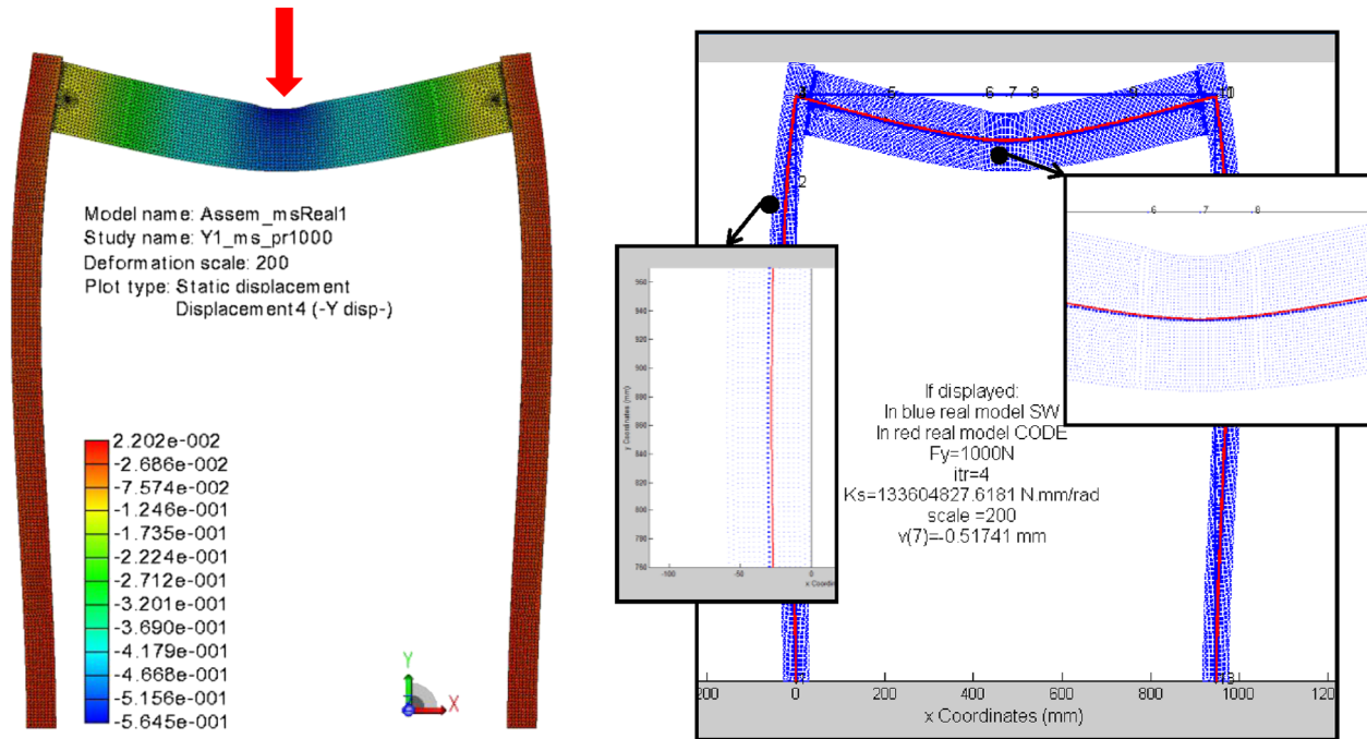
Fig. 5. Comparison between the displacement field of the mean line of the 3D FEA and the “beam + spring” one.
