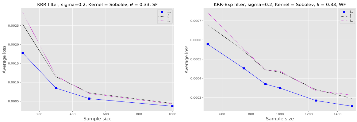
Figure 2: We choose Sobolev kernel, noise level \sigma = 0.2 and apply KRR (linear parameterization) and KRR (exponential parameterization) filters with \alpha = 0.5 for (SF) and (WF) regression functions. Smoothing parameter \theta is chosen to be equal to inverse estimation of the decay of the eigenvalues of Gram matrix. Each curve for both of two graphs corresponds to the mean-squared error of a spectral filter estimator, stopped at t_{\text{or}} , t_w and \hat{t} , averaging over 100 independent trials.
