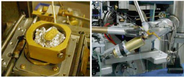
Figure 1. (a) Cartouche finger-ring in the sample-holder of the SEM; (b) fibula during PIXE analysis at AGLAE (© M.F. Guerra, C2RMF)
