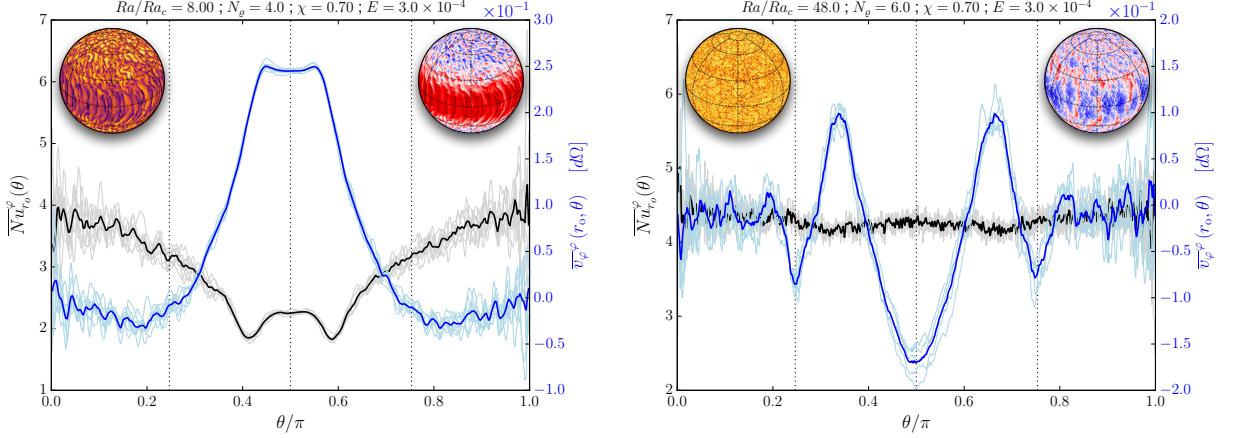
Fig. 1. Nusselt (black) and zonal velocity (blue) profiles as a function of colatitude for different thin shell models. The color insets represent snapshots of S(r = 0.98r_o) and v_\varphi(r = r_o) . The positions of the equator and the tangent cylinder are indicated by vertical dotted lines.
