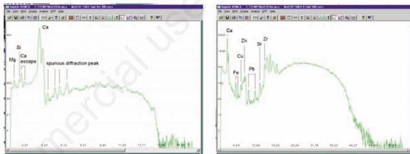
Figure 2. X-ray spectra of major elements (Mg, Ca) and trace elements (Fe, Cu, Zn, Sr, Pb).
