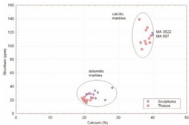
Figure 3. Strontium vs calcium plot discriminating calcitic and dolomitic marbles.
