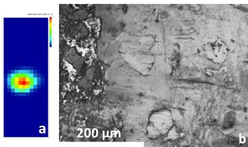
Fig. 7. (a) Elemental distribution by \mu PIXE in colour scale of the Ir ( L\alpha -line) in an area shown under the SEM (b) of the cartouche E7168 cover sheet containing PGE inclusions.
