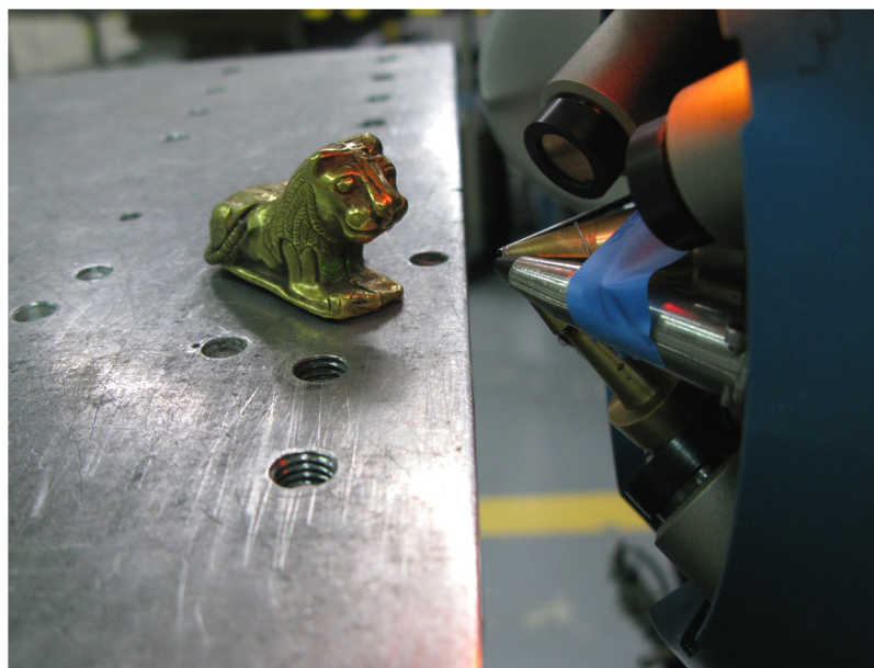
Fig. 2. One of the gold lions from King Ahmose's armband E7168 during \mu PIXE analysis at the extracted beam line of the AGLAE accelerator facility (C2RMF).
