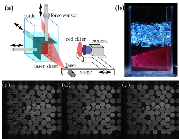
Fig. 1 a Schematic view of the experimental set-up. A stage holding a camera equipped with a red filter and a laser creating a red light sheet is translated to scan a tank containing index-matched liquid and polyacrylamide beads that are loaded with three plates moving along three orthogonal axes. b View of the polyacrylamide beads (top) in the index-matched liquid (bottom). The tank is partially illuminated with a laser sheet. Reprinted from Rev. Sci. Instr. 83 , 011301 (2012), with the permission of AIP Publishing. c , d , e Evolution (from left to right) of the view of a slice in the middle of the tank with increasing Polyvinylpyrrolidone (PVP) concentration, which is gradually added to index-match the liquid surrounding the particles (color figure online)
