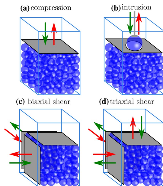
Fig. 2 Schematic view of the different experimental loading mechanisms: a uniaxial compression of monodisperse and bidisperse grains; b intrusion of a large sphere in monodisperse grains; c isochoric biaxial shearing; d isochoric triaxial shearing. Green arrows stand for the displacement during the forward part of the loading while red arrows stand for the backward part (color figure online)
