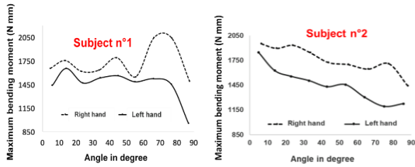
Figure 2: Changing of the maximum bending moment versus the angle of articulation for different subjects
