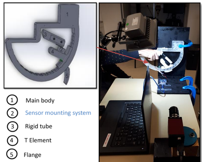
Figure 1-Laboratory set-up developed for the experimental investigations
