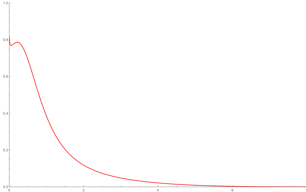
Figure 8: The density function for Av(1324) constructed numerically.
