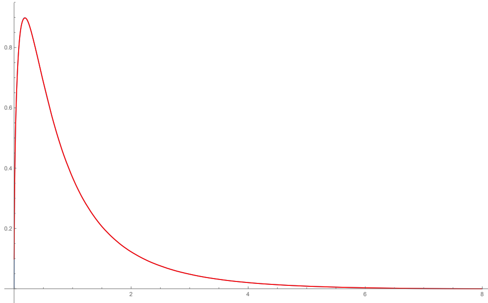
Figure 2: The density function for Av(1342) constructed numerically, and a plot of the exact expression.
