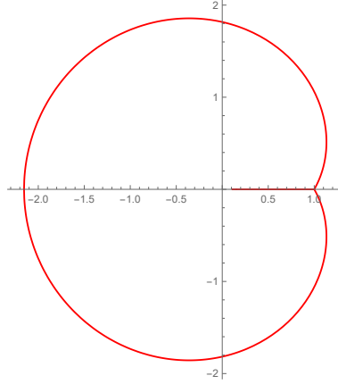
Figure 10: The cuts of the functions f_2(x) and \mathcal{H}_2(x) .
