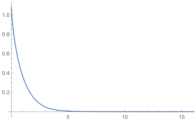
Figure 4. The density function for Av(12345) from the exact expression.
