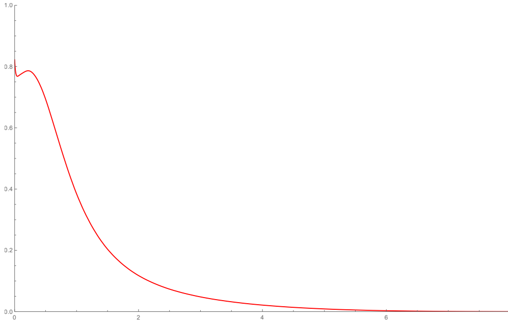
Figure 6. The density function for Av(1324) constructed numerically.
