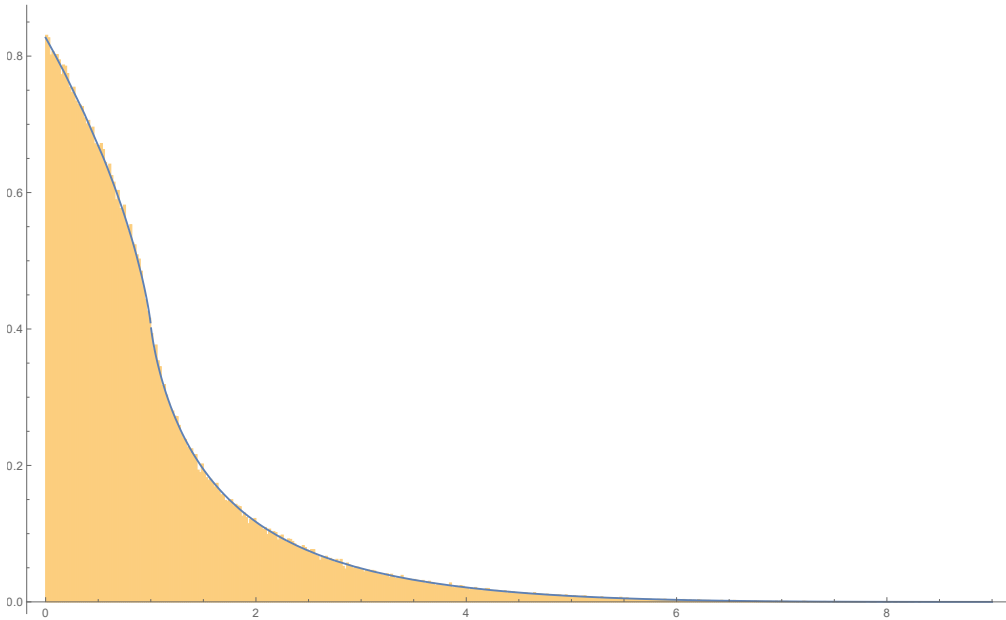
Figure 3. The density function \mu_3(x) for Av(1234) constructed numerically, and a plot of the exact expression.
