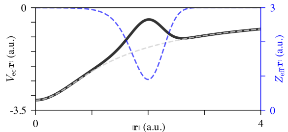
FIG. 2: Effective potentials for the ion-electron interaction as a function of the distance from the ionic core. The black vertical axis on the left refers to the electron-core potential V_{\text{ec}}(\mathbf{r}) , and the blue (gray) vertical axis on the right refers to the effective charge Z_{\text{eff}}(\mathbf{r}) , which is given by Eq. (6) and represented by the dashed blue (dark gray) line. The ion-electron potential is given by Eq. (5), and represented by the solid black line. The soft-Coulomb potential V_{\text{ec}}^{(\text{SC})}(\mathbf{r}) is given by Eq. (5) and represented by the dashed light gray line.
