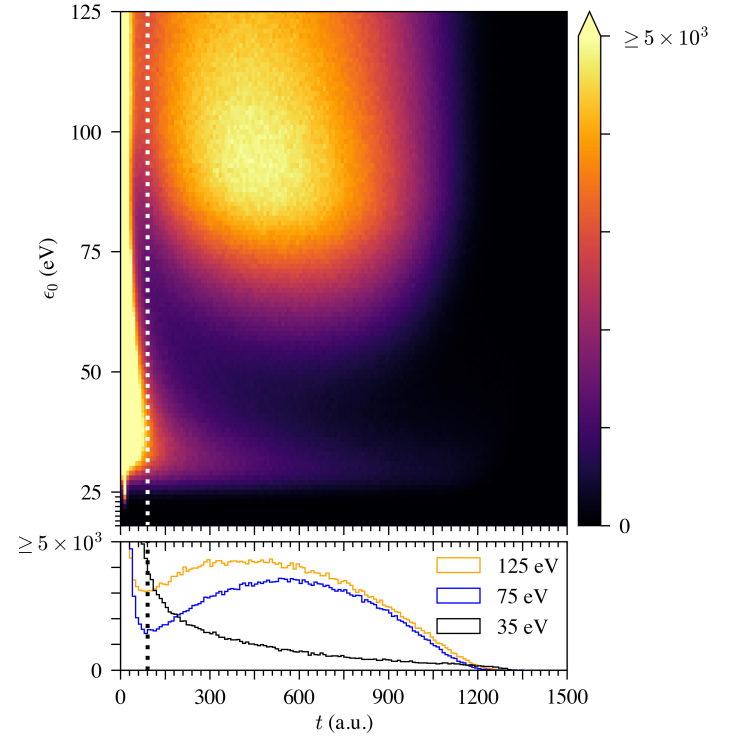
FIG. 4: Upper panel : The distribution of times when the last ionization occurs in the double ionization process as a function of the impact energy, \epsilon_0 . We say that the last ionization occurs when the last ionized electron crosses |\mathbf{r}| = 8 a.u. The time intervals along the horizontal axis are 10 a.u. wide. The color-bar indicates the count of total double ionizations for the corresponding \epsilon_0 and ionization time. Lower panel : The distribution in times of the initiation of the last ionization for \epsilon_0 equal to 35 eV in black, 75 eV in blue (dark gray) and 125 eV in orange (light gray). The vertical axis measures the count of double ionizations. The time intervals along the horizontal axis are 10 a.u. wide. The dotted vertical line indicates t_{Th} = 90 a.u.
