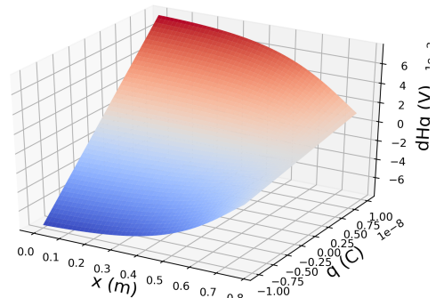
Fig. 7. Constitutive law of the variable capacitor.
