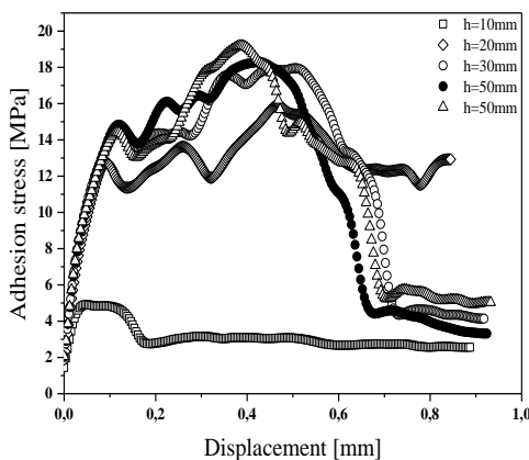
Figure 6: Stress-displacement relationship for different concrete cover.
