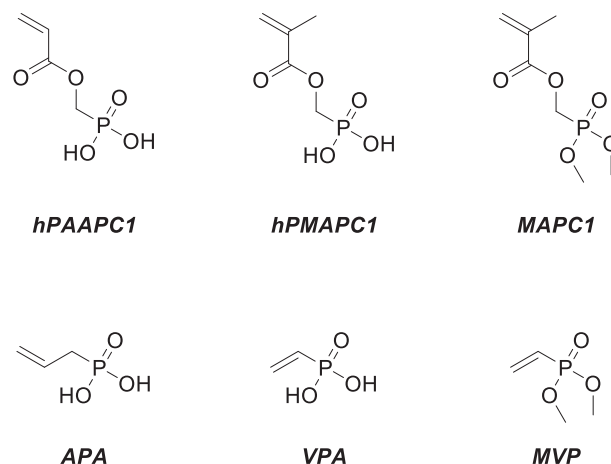
Fig. 1. Phosphorus-based molecules used in this study.
