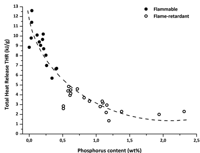
Fig. 13. Total heat release (PCFC) and flammability of flax fabrics in function of phosphorus content (dotted line is only guideline for eyes).
