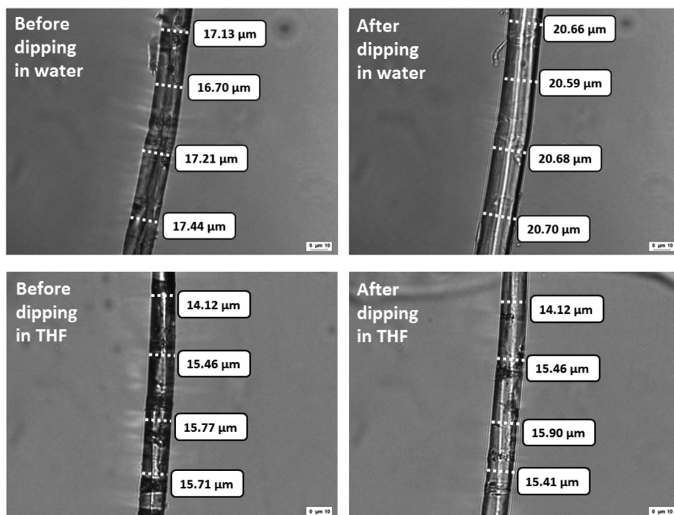
Fig. 6. Influence of water and THF on the diameter of flax elementary fibers.
