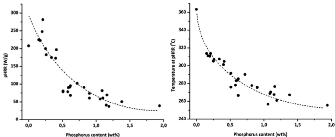
Fig. 11. Influence of phosphorus content on the intensity of the peak of heat rate release and its corresponding temperature under anaerobic pyrolysis (dotted lines are only guidelines for eyes).
