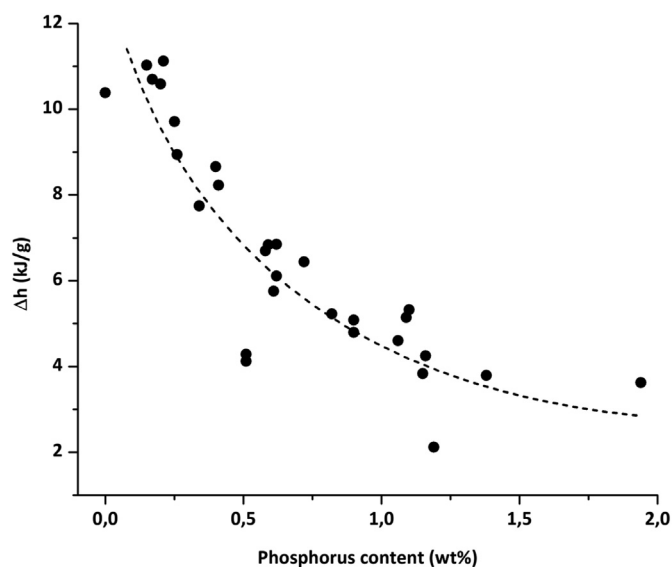
Fig. 10. Influence of phosphorus content on the heat of complete combustion ( \Delta h ) of flax fibers (dotted lines are only guidelines for eyes).
