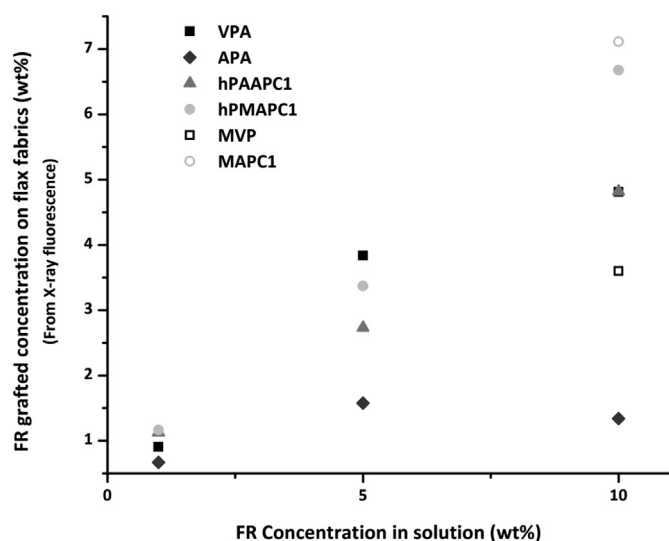
Fig. 3. FR grafted concentration on flax fabrics (from X-ray fluorescence) at different concentrations in aqueous solution irradiated at a dose of 50 kGy and washed by water.
