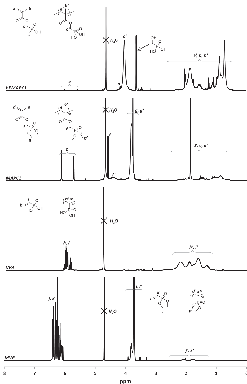
Fig. 8. ^1\text{H} NMR spectra of hPMAPC1, MAPC1, VPA and MVP irradiated at 50 kGy.
