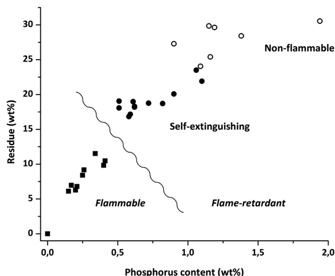
Fig. 12. Char yield versus phosphorus content obtained from fire test.
