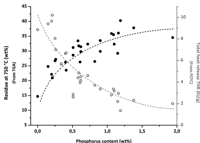
Fig. 9. Influence of phosphorus content on residue content using TGA and total heat release using PCFC (dotted lines are only guidelines for eyes).
