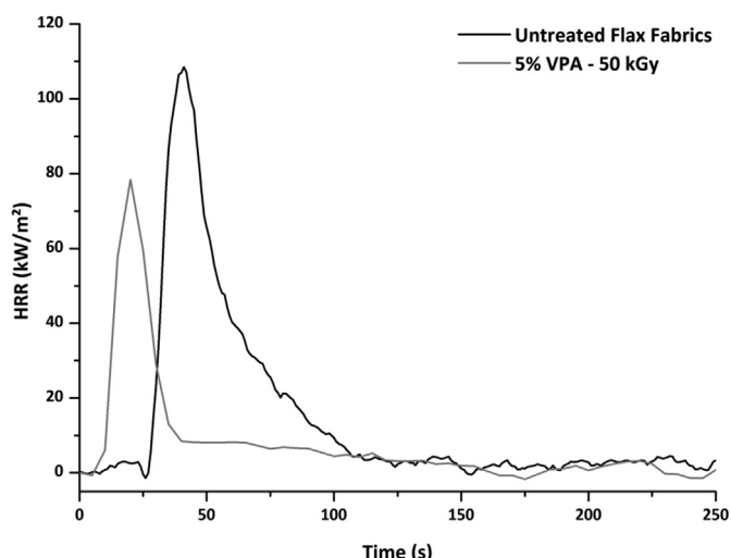
Fig. 14. HRR curves at heat flux of 35 kW/m 2 for untreated flax fabrics and for modified fabrics with a solution of 5 wt% of VPA and irradiated at 50 kGy.
