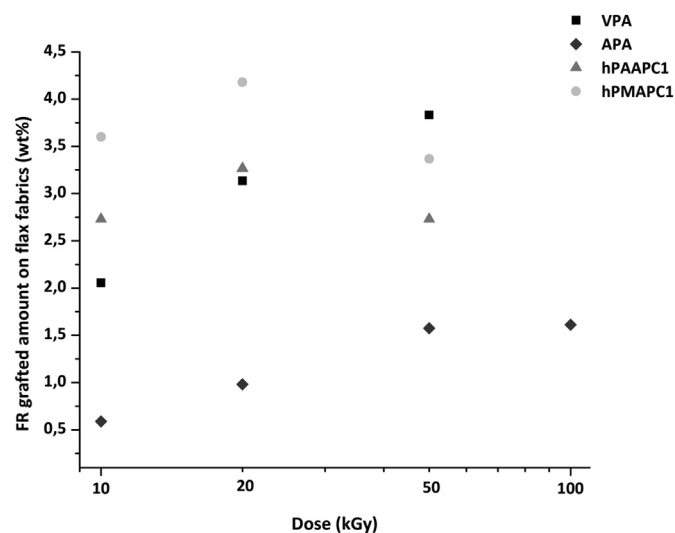
Fig. 4. Influence of radiation dose on grafted FR amount for flax fabrics impregnated with a solution containing 5 wt% of the FR monomer, irradiated and washed with water.
