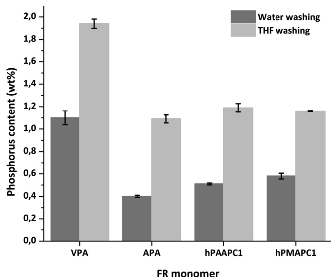
Fig. 5. Influence of the choice of the washing solvent on final phosphorus content (monomers concentration in solution = 5 wt%; radiation dose = 50 kGy).
