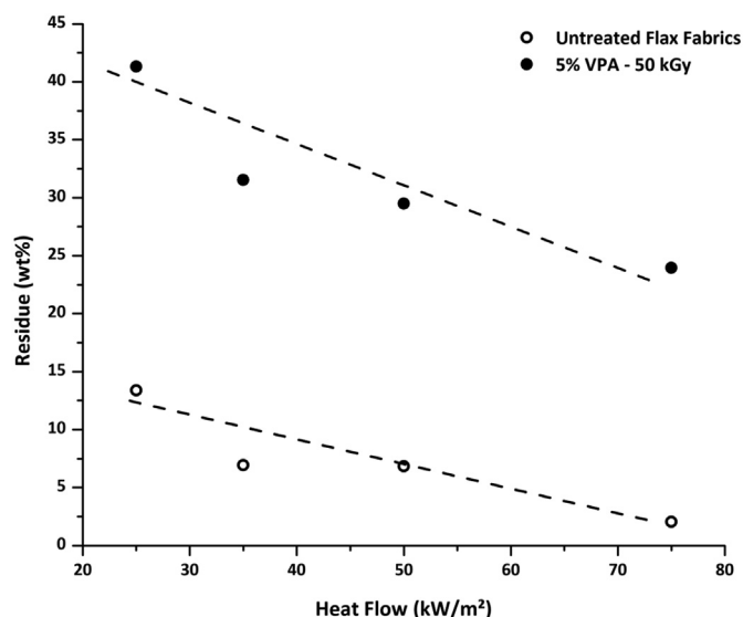
Fig. 15. Evolution of the percentage of residue as a function of the heat flux (The dotted lines are only indications for the eyes).
