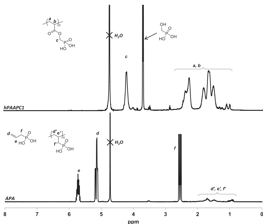
Fig. 7. ^1\text{H} NMR spectra of hPAAPC1 and APA dissolved in water and irradiated at 50 kGy.
