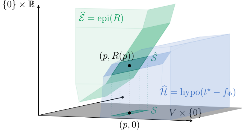
FIGURE 1. The solution set \mathcal{S} is equivalent, up to an affine isomorphism, to the set \hat{\mathcal{S}} (see Lemma 1).
