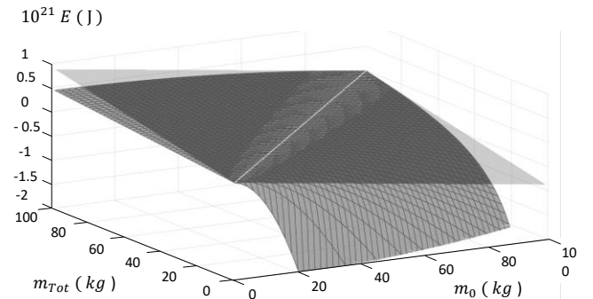
Figure 4. Differences between equations (40) and (51)
