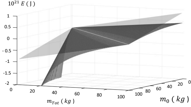
Figure 5. Differences between equations (40) and (51)
