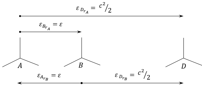
Figure 1. Specific energy differences of the particles and their associated reference frames
