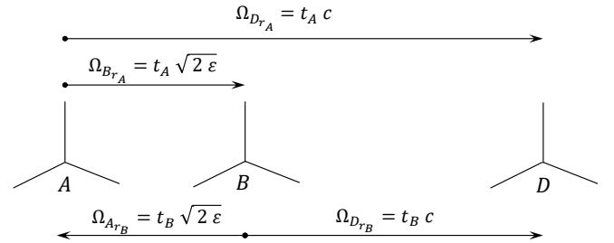
Figure 2. Equivalent distances between the particles and their associated reference frames
