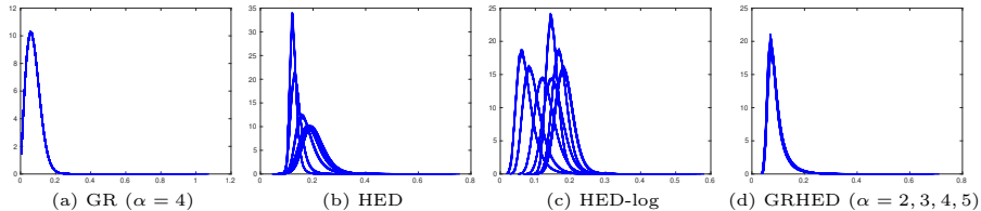
Figure 15: The histograms of the gradient magnitude fields produced by GR, HED, HED-log and GRHED in 160 1-look pure noise images of size 1024 \times 1024 pixels. There are 8 possibilities for the square root of the mean intensity values of these images, namely, 50, 80, 120, 150, 180, 200, 230 and 250. For noise images with each mean intensity value, there are 20 random realizations.
