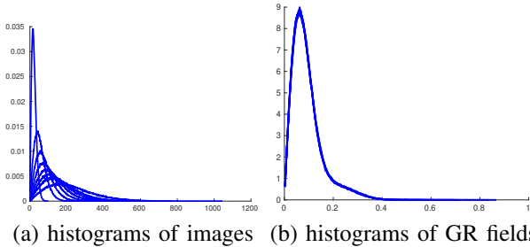
Fig. 3: Histograms of the eight 1-look synthetic edge images and histograms of their gradient magnitude fields computed by GR with \alpha = 4 .
