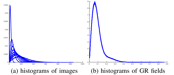
Fig. 4: Histograms of the eight 1-look synthetic edge images and histograms of their gradient magnitude fields computed by GR with \alpha = 4 .
