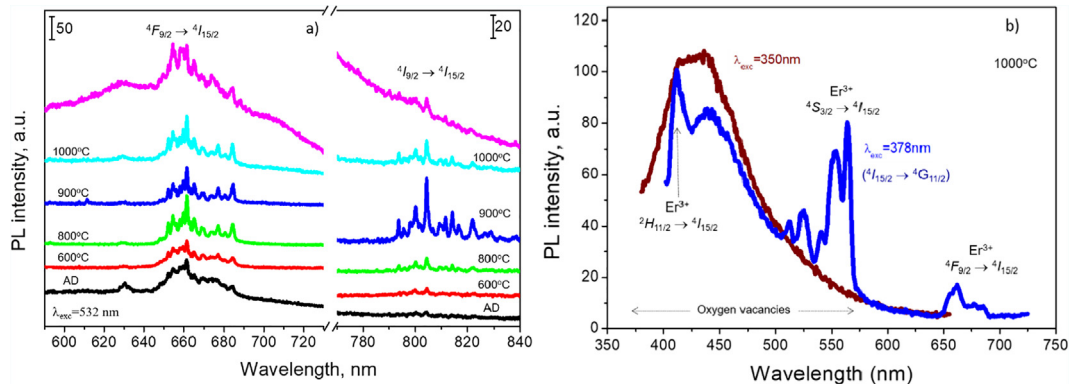
Fig. 3. a) Evolution of PL spectra of \text{Er}_2\text{O}_3 films with T_A . Excitation light wavelength is 532 nm. The spectra are shifted in vertical direction for clarity. b) PL spectra of the film annealed at 1000 °C recorded under non-resonant (350 nm) and resonant (378 nm) excitations.
