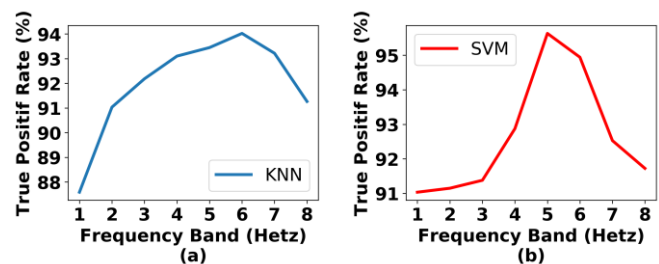
Fig. 3. TPR According to the Frequency Band of Calculated MFCC.
