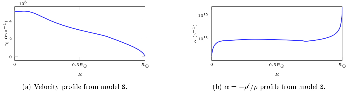
Figure 1: Profiles of the solar parameters with the model S. In our analysis, we consider the scaled velocity c_0 = c_0/R_\odot , given in terms of the scaled radius r = R/R_\odot .
