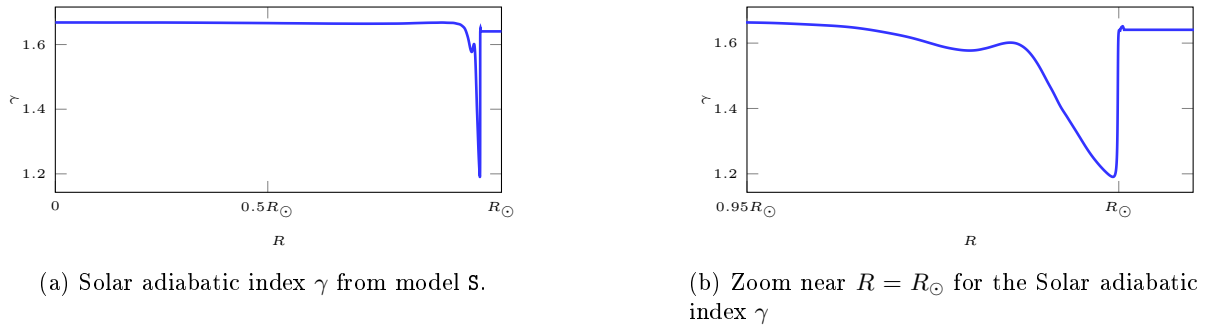
Figure 3: Adiabatic index profile extracted from the solar model S.
