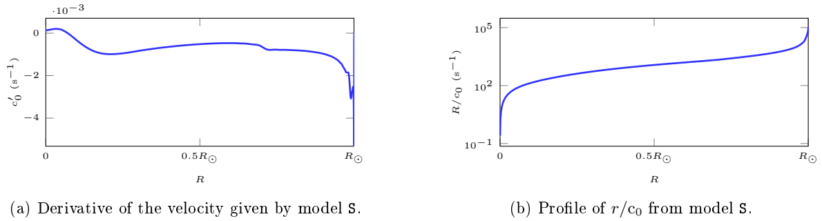
Figure 2: Quantities used for the analysis associated with the solar model S. In our analysis, we consider the scaled velocity c_0 = c_0/R_\odot , given in terms of the scaled radius r = R/R_\odot , therefore, we have R/c_0 = r/c_0 .
