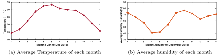
Fig. 2. Average temperature and humidity of Delhi-NCR monthwise during the 2018 civil year
