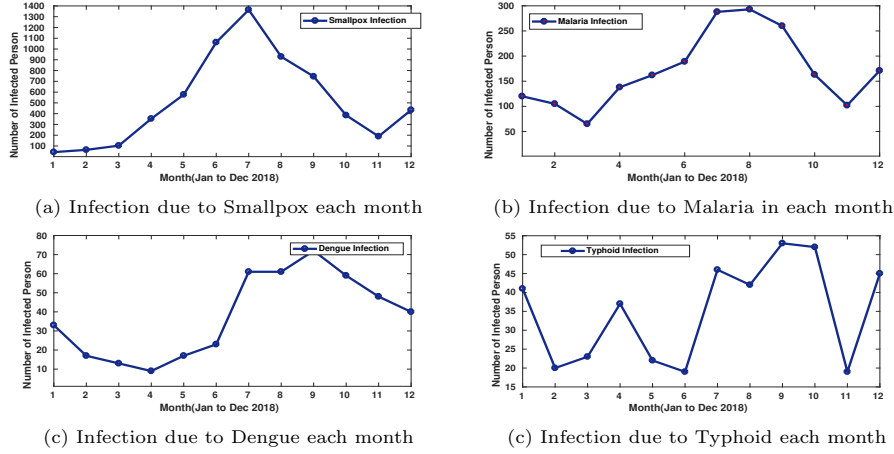
Fig. 1. Number of infected persons each month recorded at Al-shifa Hospital New Delhi for various diseases during the 2018 civil year
