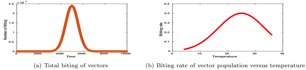
Fig. 6. Biting of vector population
