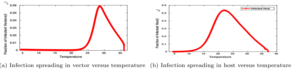
Fig. 7. Effect of Temperature on infection spreading in vector and host populations
