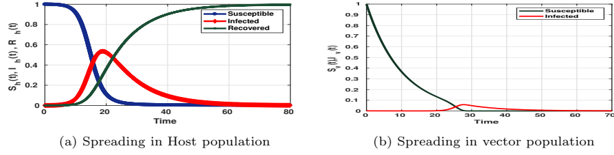
Fig. 4. Epidemic Spreading in Host and Vector Population
