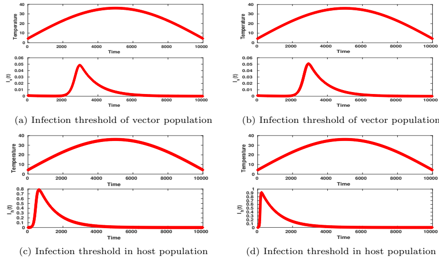
Fig. 5. Effect of temperature on infection threshold in SIR considering a homogeneous contact network
