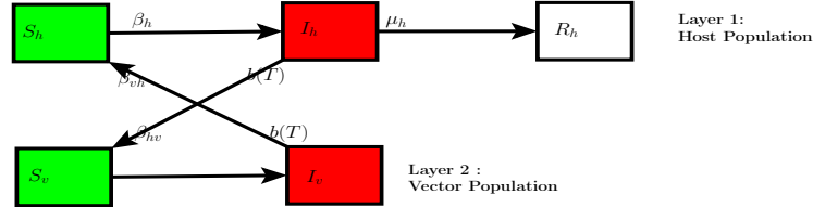
Fig. 3. Block diagram of the proposed model incorporating the temperature influence on the biting rate
