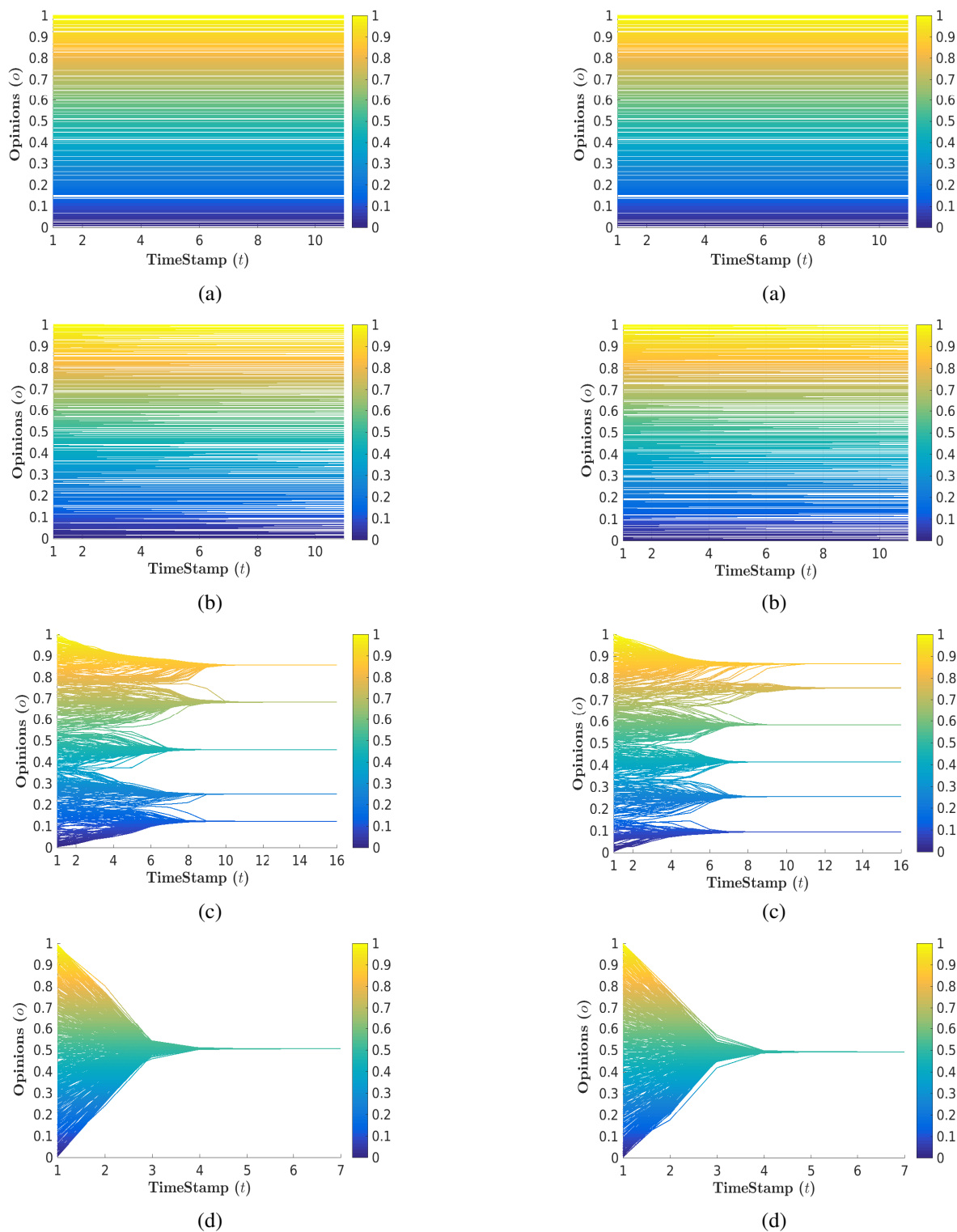
FIGURE 2. Evolution of opinion of the respective nodes versus timestamp until get convergence. The fraction of the top ranked nodes ( \beta ) fixed at 0%. The centrality used to weight the opinions is Page Rank on network of size 500. Different values of the threshold ( \alpha ) are considered as (a) No Convergence with \alpha = 0 (b) Convergence with \alpha = 0.004 (c) Convergence with \alpha = 0.08 (d) Consensus with \alpha = 0.5 . Different colors represent different opinion values in the range [0, 1] .
