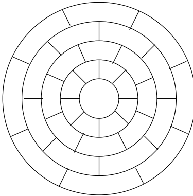
Figure 1: The m -barrel fullerene F(8, 2) .
