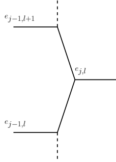
Figure 4: Labeling of the horizontal edges of F(m, k) .
