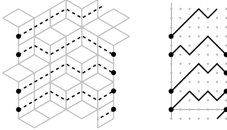
Figure 5: Conversion of the rhombic tiling (left) to a family of non-intersecting paths (right). Notice how the path starting from the left topmost starting point winds around the cylinder to connect to the bottom most ending point on the right.
