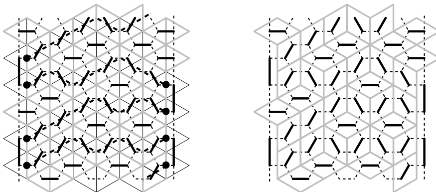
Figure 3: The correspondence between perfect matchings on F(6,5) (left) and rhombi tiling on the cylinder. Recall that the graph is drawn on a cylinder, so that the edges at the top are connected to vertices at the bottom.
