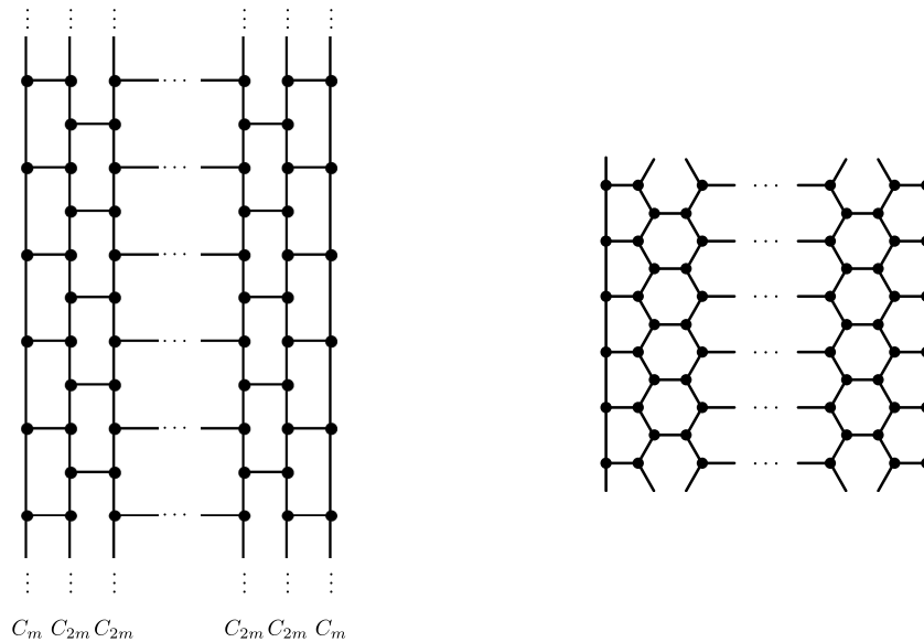
Figure 2: Left: an m -barrel fullerene, represented on the cylinder. The top and bottom are identified to create the cylinder. The cycles C_m on the extremities are the boundary of the cylinder and correspond to the boundaries of the m -gons in the representation of Figure 1. Right: the same graph on the cylinder, slightly deformed so that hexagonal faces are regular.
