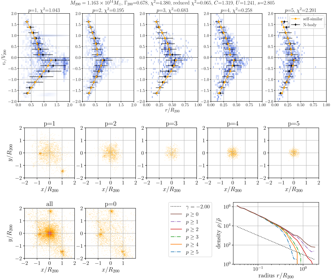
Figure 6. Same as in Fig. 5, but for a slightly less massive halo with M_{200} = 1.163 \times 10^{14} M_{\odot} . This is the same halo as shown in the second from the top in Fig. 3.
