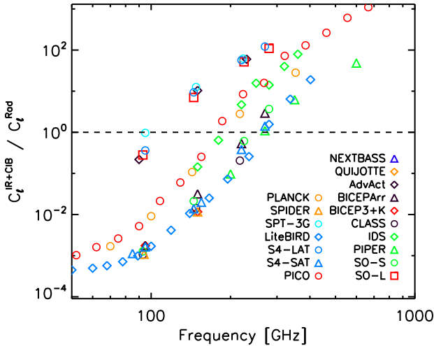
Fig. 5. Ratio between the BB power spectra of [IR shot noise + clustering] and radio shot noise, at \ell=80 for all CMB experiments.
