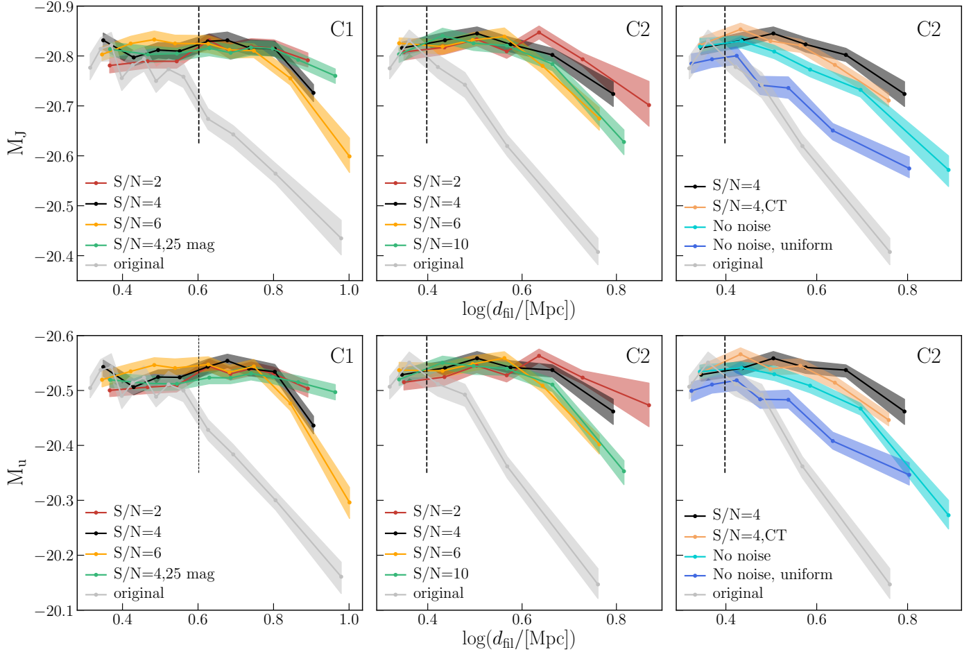
Fig. 7. Distributions of the mean M_J (top) and M_u (bottom) galaxy rest-frame magnitudes as a function of the distance to the filaments ( d_{\text{fil}} ) for galaxies with \log M_{\star}/M_{\odot} > 9.0 . Results are shown for the C1 (left column) and the C2 (middle column) configurations. Right column: additional flavours of the C2 configuration (see Sect. 2.1.4 and the caption of Fig. 4 for details). The vertical dashed line indicates the reconstruction scales L_T of 4 and 2.5 Mpc for the C1 and C2 configurations, respectively. Below this scale, no trend is expected towards the reconstructed filaments.
