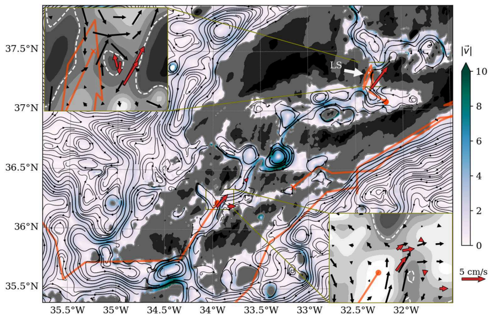
FIGURE 2 | Rift valley circulation at 2,000 m. The mean flow from numerical modeling is shown in black (“streamplot” with the line thickness proportional to the speed amplitude) and colors further indicate its magnitude. Superimposed are two ARGO float tracks near 1,990 m inside the rift valley and two other ones near 1,500 m flowing southward along the eastern flank of the ridge (orange, with the location of the release and last record indicated by a plain circle and a cross, respectively). Red arrows represent the mean velocity from selected moorings near the Rainbow vent field (2,100 m deep) and in the East canyon at Lucky Strike (1,875 m, LS label). Insets show zooms over these regions, representing the mean flow with black arrows. Black shading indicates bathymetry (using the same convention as in Figure 1 ) and white dashed contours in the insets indicate the depth at which the mean velocity is computed from the simulation (2,100 m at Rainbow, 1,800 m at Lucky-Strike, to match most of the available observations). At Rainbow, all 6 moorings available in the region are plotted. At Lucky-Strike, moorings are taken from (going west to east): Momar (1,700 m), DIVA (1,680 m), and Graviluck (1,930 and 1,874 m).
