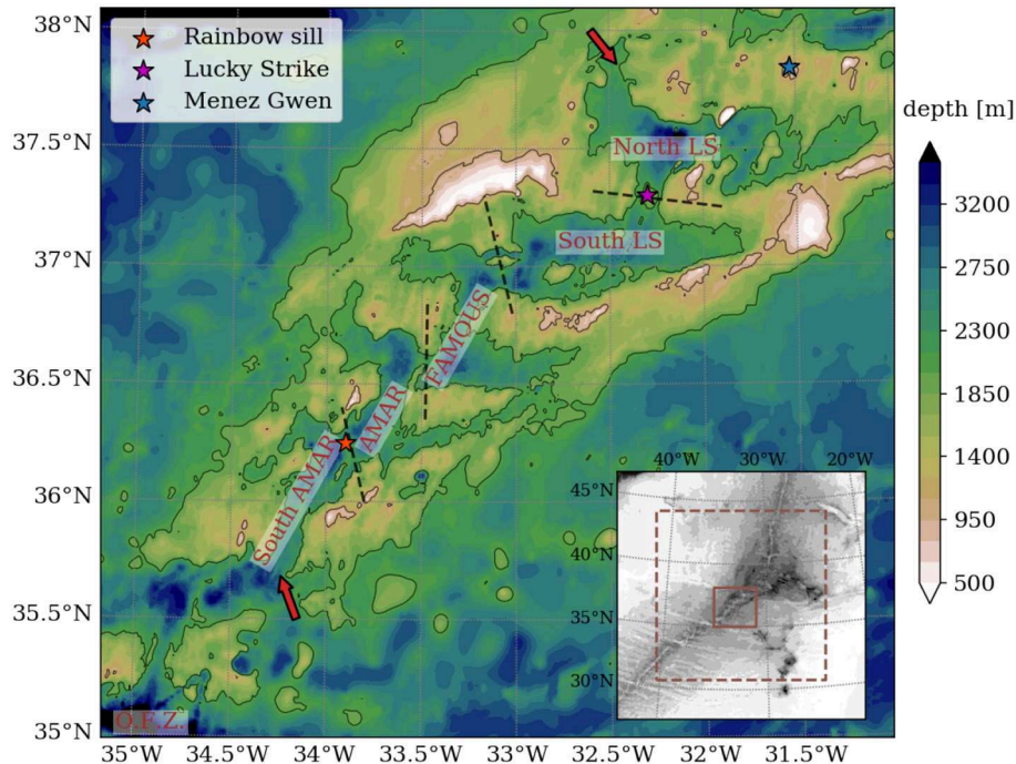
FIGURE 1 | Bathymetry of the North Mid-Atlantic Ridge in the region discussed in this paper (taken from the SRTM30plus database). Black contours indicate iso-depth at 2,000 and 1,000 m. Dashed lines delimitate basins and segments of interest (written in brown). These are usually associated with fracture zones aligned along the West-East direction. The rift valley water is mostly isolated below 2,000 m, except at a few locations: red arrows indicate identified connections (inflows) from the exterior ridge flanks to the inside valley at some of these passages. O.F.Z., Oceanographer Fracture Zone.
