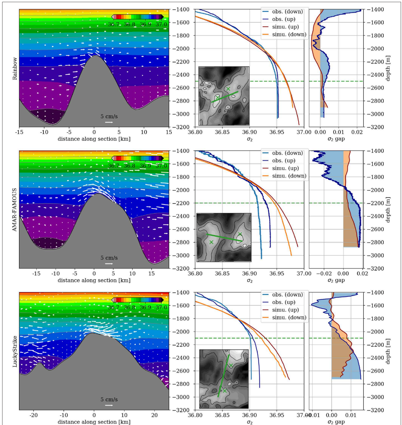
FIGURE 6 | Density changes across three prominent sills in the rift valley, namely the Rainbow sill near 36.25°N (upper row), the AMAR-FAMOUS overflow sill near 33.5°W, 36.5°N (middle row), and the Lucky-Strike segment center near 37.25°N (lower row). Left panels show mean potential density anomaly referenced at 2,000 m at vertical sections across the sill, together with the along-section component of the mean flow in white arrows. Location of the sections are indicated by green lines on the mapped bathymetry (gray) shown in the middle panels. Middle column: upstream (darker) and downstream (lighter) potential density vertical profiles from CTD stations (blue shade) and from the numerical simulation (red shade—3-month average). The location of the profiles are indicated by green crosses in the inset maps of the middle panels. The dashed green horizontal line indicates the maximum depth of the sill. Right column: upstream—downstream potential density difference. The CTD profiles at the AMAR-FAMOUS passage are taken in 2007 (MOMARdream cruise) and are very similar to equivalent profiles in 1997 (Thurnherr and Richards, 2001, Figure 7A).
