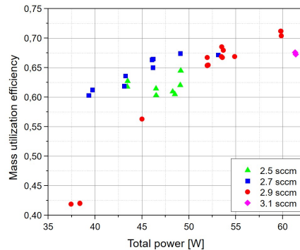
Figure 10: Mass utilisation efficiency as a function of the total power at different xenon flow rates.
