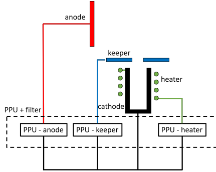
Figure 3: Schematic of the electrical connections between anode, cathode and PPU.
