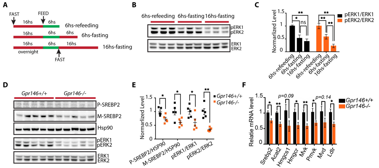
Figure 5. GPR146 Regulates ERK/SREBP2 Axis in Mice upon Short Period of Fasting (A) Schedule of fasting and refeeding treatment in vivo . (B and C) Western blot (B) and relative quantification (C) of phosphorylated ERK1/2 (pERK1/2) and total ERK1/2 in livers of mice upon different fasting refeeding regimens (n=3 mice per group, by one-way ANOVA). (D and E) Western blot (D) and relative quantification (E) of SREBP2 precursor (P-SREBP2), mature SREBP2 (M-SREBP2), pERK1/2 and total ERK1/2 in livers of 6-hour fasted Gpr146 +/+ mice and Gpr146 -/- littermates (n=5 mice per group, by Student's t -test). (F) Quantitative polymerase chain reaction (qPCR) expression analysis of cholesterol biosynthetic genes in liver of 6-hour fasted Gpr146 +/+ mice and Gpr146 -/- littermates (n=5 mice per group, by Student's t -test). * p < 0.05 , ** p < 0.01 ; bars in C and E indicate mean \pm s.d., bars in F indicate mean \pm s.e.m..
