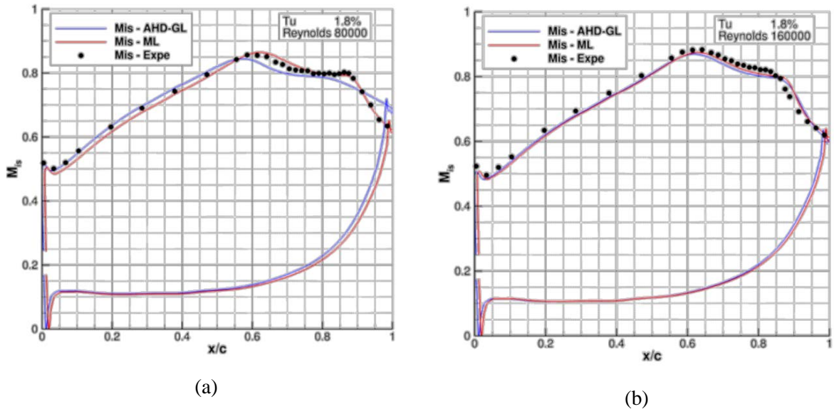
Figure 10.10 : Results obtained for the T106C turbine blade (blue lines: transition criterion approach, red lines: \gamma - \overline{R_{\theta_T}} approach, symbols: experiments)
