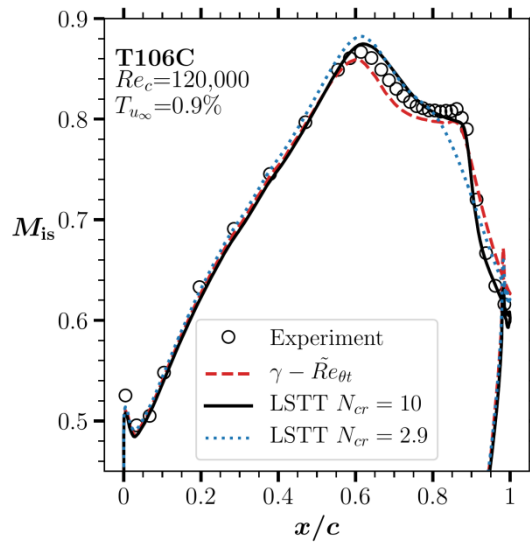
Figure 10.11 : T106C result at Re 120000 (LSTT & \gamma - \overline{R_{\theta_T}} )
