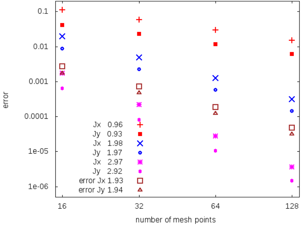
Figure 7: Theoretical and measured rates of convergence \theta for classical bounce back (9) as a function of the number of mesh points in the axial direction. The error is proportional to \Delta x^\theta in the \ell^2 norm for x and y component of the momentum, for aspect ratio \frac{L}{h} = 2 .
