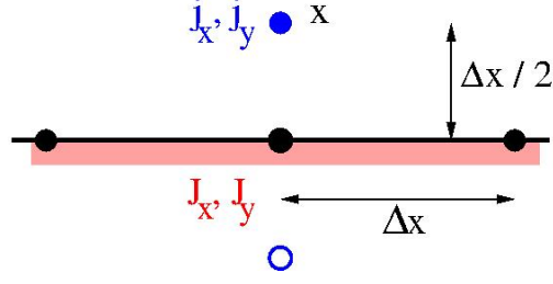
Figure 4: Expansion of the momentum (j_x, j_y) in the first cell as a function of the data (J_x, J_y) on the boundary.
