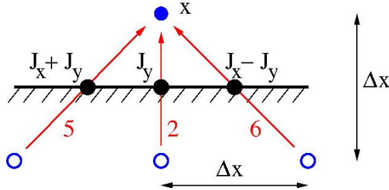
Figure 6: Approximation of the momentum gradient with finite differences.
