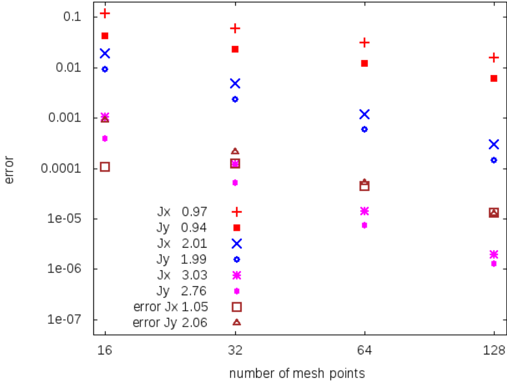
Figure 8: Theoretical and measured rates of convergence \theta for generalized bounce back (40) as a function of the number of mesh points in the axial direction. The error is proportional to \Delta x^\theta in the \ell^2 norm for x and y component of the momentum, for aspect ratio \frac{L}{h} = 2 .
