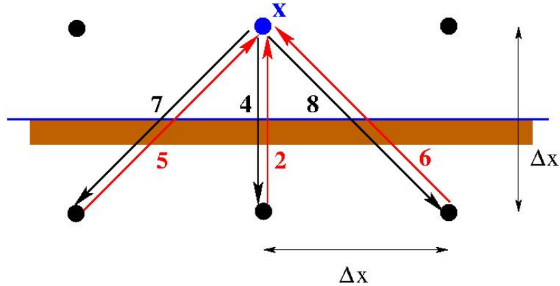
Figure 3: Bounce back scheme for bottom boundary configuration with the D2Q9 scheme.
