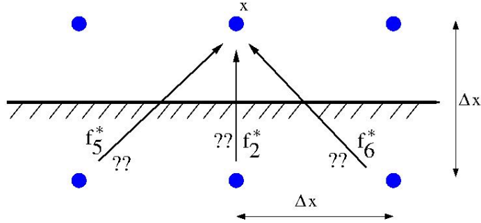
Figure 2: Missing distribution functions to define the boundary scheme for the D2Q9 on a boundary located at y = 0 .
