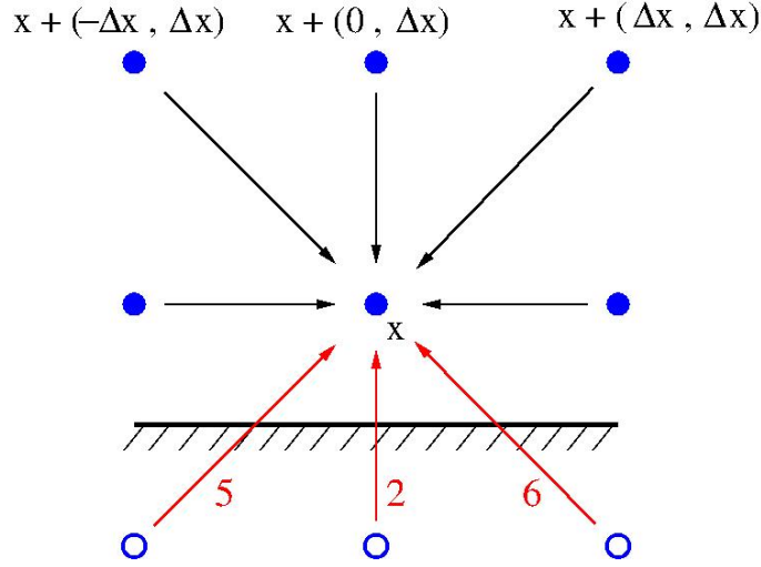
Figure 5: Node near the boundary for the D2Q9 scheme.
