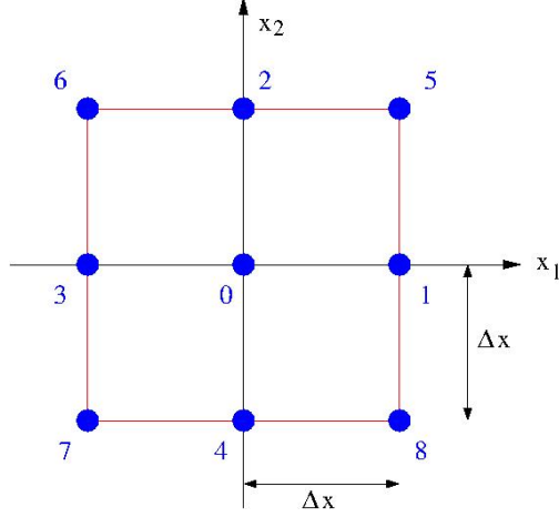
Figure 1: Particle distribution f_j for 0 \leq j \leq 8 of the D2Q9 lattice Boltzmann scheme.
