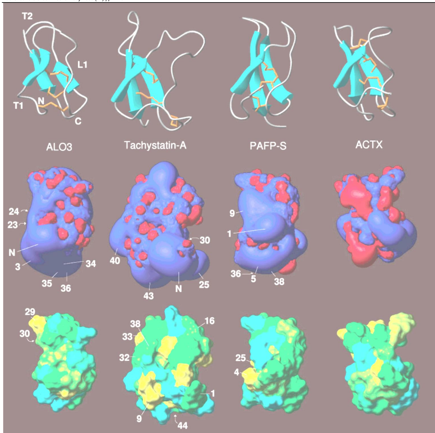
Figure 5: (Top) Global fold of Alo-3, tachystatine A, PAFP-S, and ACTX. (Middle) Electrostatic contours at +1 \text{ e } \text{\AA}^{-1} (red) and -1 \text{ e } \text{\AA}^{-1} (blue) for the four molecules in the same orientation and in the same order. (Bottom) Distribution of hydrophobic and hydrophilic residues at the surface of the four molecules according to the hydrophobic scale of Eisenberg (41): yellow (Val, Leu, Ile, Trp), green (Cys, Ala, Gly, Tyr, Pro, Thr, Ser, Asn, Gln), blue (His, Asp, Asn, Glu, Gln, Arg, Lys). This figure was drawn with MOLMOL (39).
