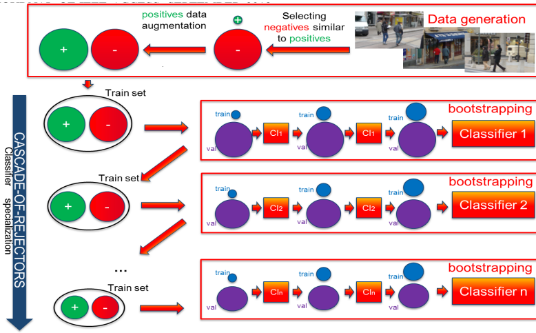
Fig. 1. Training pipeline. The initial training set generation selects data while balancing negative and positive sample cardinalities (Top). A cascade classifiers is then trained on it (Left), each independent classifier being learnt through bootstrapping (right). balanced positive and negative sets is sought all along the cascade. c_i :classifier
