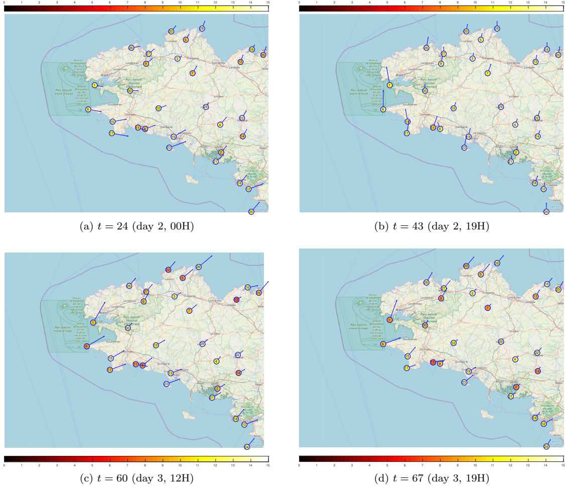
Figure 4: Visualization of some snapshots of Molène Dataset. Each point represents a weather station (see ?? for stations' names). The blue arrows represent wind direction and their length is proportional to wind speed. The color of each station refers to the recorded temperature (in °C). The map shows the French region between 47°N and 49°N and 2°W and 6°W and was downloaded from openstreetmap.org .
