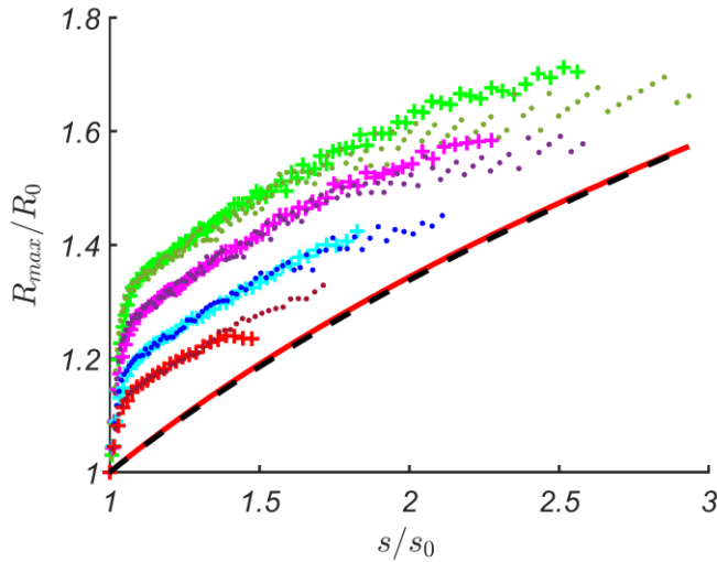
Figure 10: The ratio of maximum run-up height in the conjoined basin, R_{\max}/A and the maximum run-up height on a plane beach, R_0/A versus the wave front steepness, s/s_0 for A/h_0 = 0.057, kh_0 = 0.38 (brown points), A/h_0 = 0.086, kh_0 = 0.38 (red plus signs), A/h_0 = 0.057, kh_0 = 0.29 (blue points), A/h_0 = 0.086, kh_0 = 0.29 (turquoise plus signs), A/h_0 = 0.057, kh_0 = 0.22 (violet points), A/h_0 = 0.086, kh_0 = 0.22 (pink plus signs), A/h_0 = 0.057, kh_0 = 0.19 (dark green points), A/h_0 = 0.086, kh_0 = 0.19 (light green plus signs). All markers correspond to the results of numerical simulations, while the asymptotic analytical predictions are given by the red solid line. Black dashed line corresponds to the power fit of the analytical results Eq. (16).
