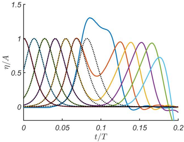
Figure 9: Wave evolution at different locations x/\lambda = 0, 0.85, 1.71, 2.56, 3.41, 4.27 and 5.12 along the section of constant depth for a basin with X_0/\lambda = 5.12 and \tan \alpha = 1:20 . Numerical results are shown by solid lines, while the analytical predictions are given by the black dotted lines. The parameters of the wave: A/h_0 = 0.03, kh_0 = 0.19 .
