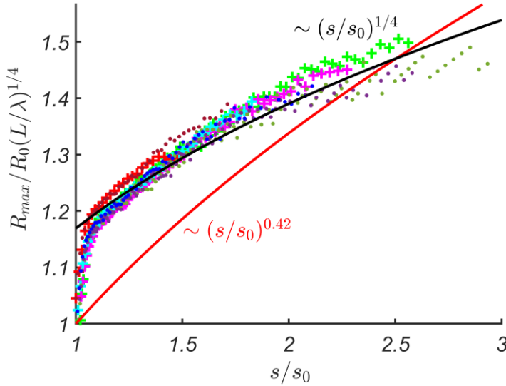
275 Figure 11: The normalized maximum run-up height R_{\max}/R_0 (L/\lambda)^{1/4} calculated numerically versus the wave front steepness, s/s_0 for the same values of A/h_0 and kh_0 as in Figure 10. Red solid line is proportional to the “analytically estimated” Eq. (16), while black solid line corresponds to Eq. (17).
