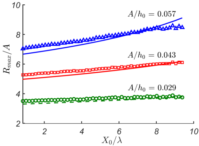
200 Figure 5: Maximum run-up height, R_{\max}/A , as a function of distance to the slope, X_0/\lambda for different amplitudes of the initial wave, A/h_0 . Analytical solution described in Section 2 is shown by lines and numerical solution described in Section 3 is shown by symbols (triangles, squares and circles) with matching colours, kh_0 = 0.38 .
