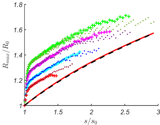
Figure 10: The ratio of maximum run-up height in the conjoined basin, R_{max}/A and the maximum run-up height on a plane beach, R_0/A versus the wave front steepness, s/s_0 for A/h_0 = 0.057, kh_0 = 0.38 (brown points), A/h_0 = 0.086, kh_0 = 0.38 (red plus signs), A/h_0 = 0.057, kh_0 = 0.29 (blue points), A/h_0 = 0.086, kh_0 = 0.29 (turquoise plus signs), A/h_0 = 0.057, kh_0 = 0.22 (violet points), A/h_0 = 0.086, kh_0 = 0.22 (pink plus signs), A/h_0 = 0.057, kh_0 = 0.19 (dark green points), A/h_0 = 0.086, kh_0 = 0.19 (light green plus signs). All markers correspond to the results of numerical simulations, while the asymptotic analytical predictions are given by the red solid line. Black dashed line corresponds to the power fit of the analytical results Eq. (16).
