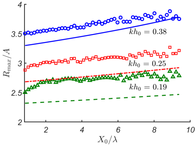
Figure 8: Maximum run-up height, R_{\max}/A as a function of the distance to the slope, X_0/\lambda for different kh_0 . Analytical solution described in Section 2 is shown by lines and numerical solution described in Section 3 is shown by symbols (triangles, squares and circles) with matching colours; A/h_0 = 0.03 .
