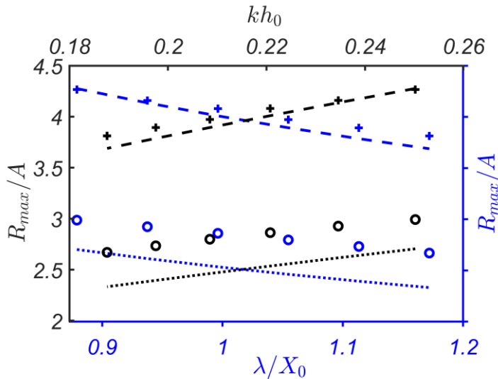
220 Figure 7: Maximum run-up height, R_{max}/A as a function of initial effective wave length, \lambda/X_0 (blue axes), and kh_0 (black axes). Analytical solutions for \tan \alpha = 1:20 and \tan \alpha = 1:50 are shown by dotted and dashed lines respectively, while numerical simulations for \tan \alpha = 1:20 and \tan \alpha = 1:50 are shown by circles and crosses respectively, A/h_0 = 0.03 .
