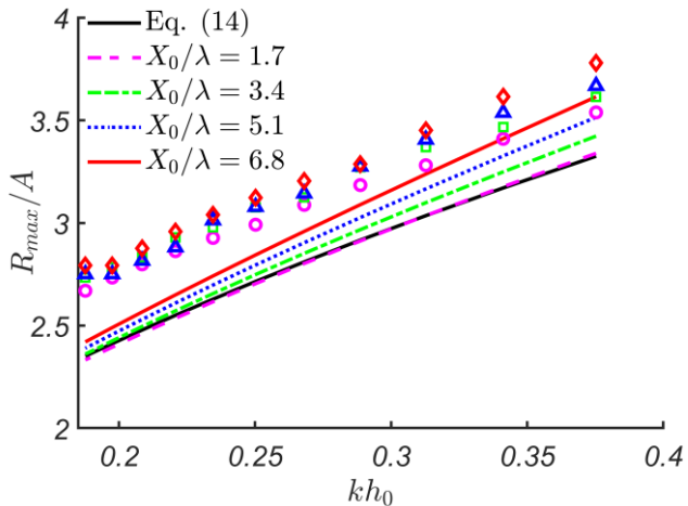
210 Figure 6: Maximum run-up height, R_{\max}/A as a function of kh_0 for different distances to the slope, X_0/\lambda . Analytical solution described in Section 2 is shown by lines and numerical solution described in Section 3 is shown by symbols (diamonds, triangles, squares and circles) with matching colours. The thick black line corresponds to Eq. (14) for wave run-up on a beach without constant depth section, A/h_0 = 0.03 .
