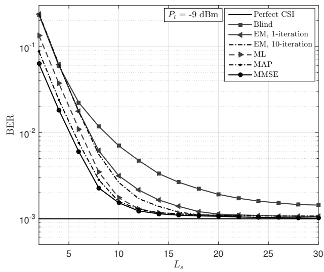
Figure 4: BER performance of EM-based, MAP, ML and MMSE estimators versus the length of the observation window L_s ; P_t = -9 dBm and the average target BER is equal to 10^{-3} .
