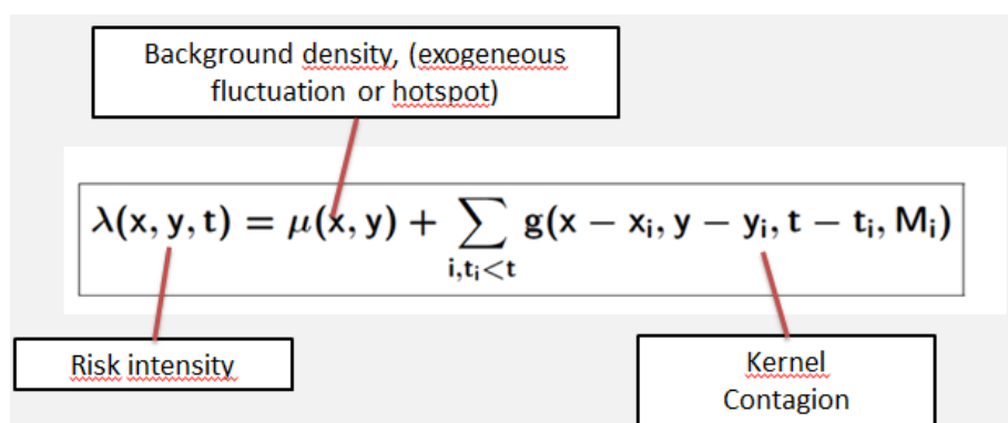
Figure 1: Predicting occurrence
