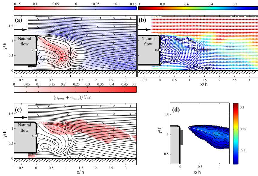
Figure 6: Natural flow characteristics in the symmetry plane ( z = 0 ), (a) Time-averaged cross-stream velocity ( \overline{v}^+ ) with the associate streamlines and the iso-line of the forward flow probability of 50%. The recirculating flow length L_\tau is also displayed by the vertical dashed line. (b) Instantaneous flow field #265 captured by the PIV. The velocity field is indicated by dimensionless norm colored arrows. The \Gamma_2 criterion is displayed by black iso-lines revealing the unforced shear-layer vortex street formation and the position of the classical main wake structures. (c) Contour map of the streamwise-transverse RMS-velocity (u_{rms} + v_{rms})/U_\infty with associated streamlines. (d) closed view of the streamwise-transverse RMS-velocity.
