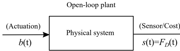
Figure 7: Sketch of open-loop control, where s denotes the sensor, herein the drag and b the actuation.
