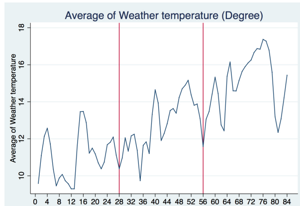
Figure 3: Daily Mean of weather temperature, ^{\circ}C
