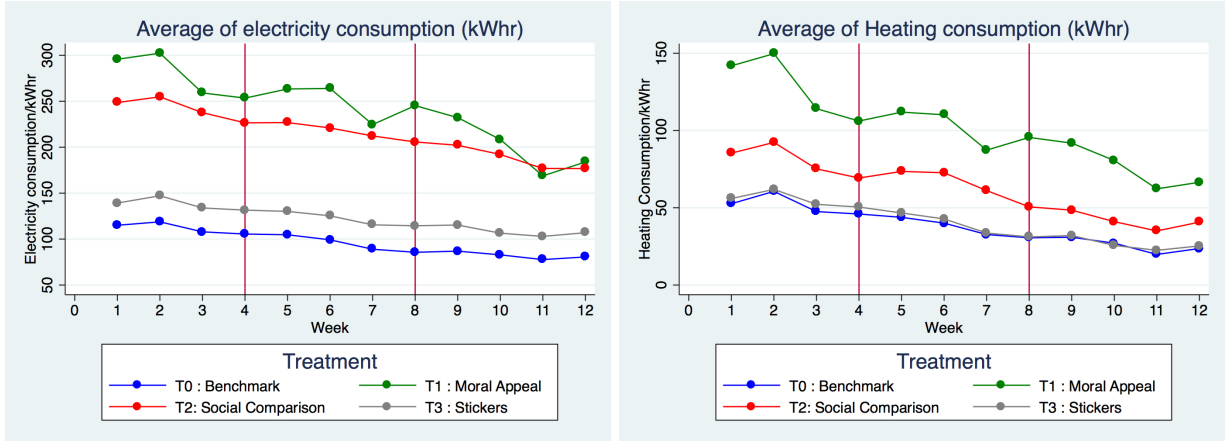
Figure 4: Mean of Electricity and Heating consumption by week
