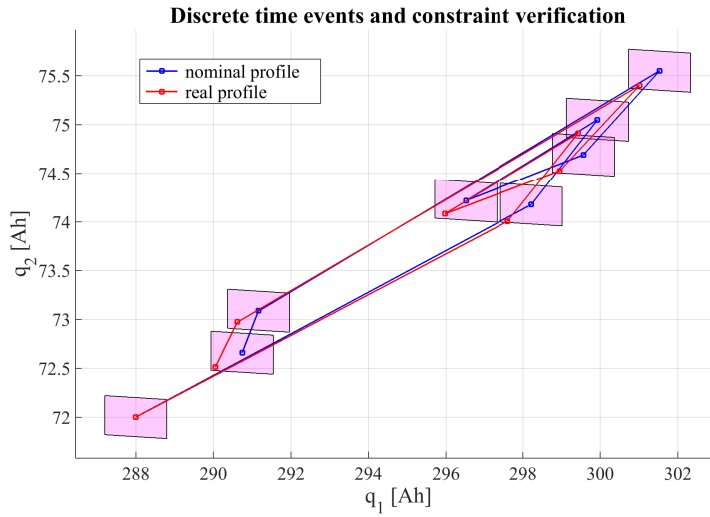
Figure 7: Ultimate bounds for discrete time events of the model states, \tilde{q}_{1b} and \tilde{q}_{2b} following the commercial use load profile.
