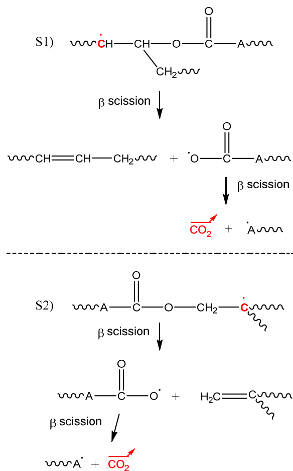
Scheme 5. Generation of volatile fragments (carbon dioxide) during the rearrangement of alkyl radicals.
